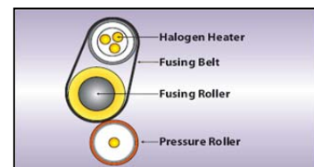
Belt fusing system consumes less power and shortens warm up time
